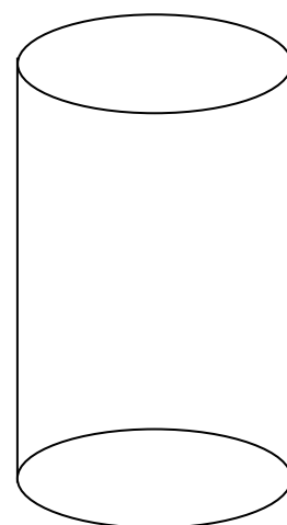
Sulfur
