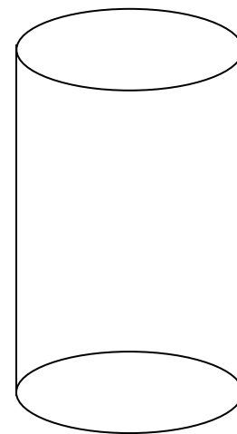
Carbon/Sulfur
