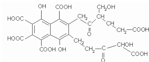
Model structure of fulvic acid
