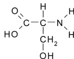
The chemical structure of a serine molecule.
