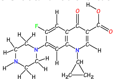
Cipro® (ciprofloxacin) 1-cyclopropyl-6-fluoro-1,4-dihydro-4-oxo-7-(1-piperazinyl)-3-quinolinecarboxylic acid
